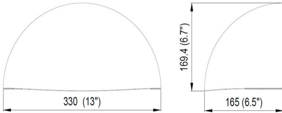
SU-WP-120W-30/40/50K-G4
