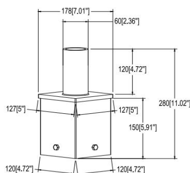
SU-SB-ACC-SQBP-2
