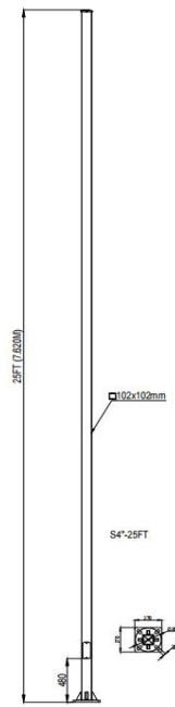
S4-25FT
