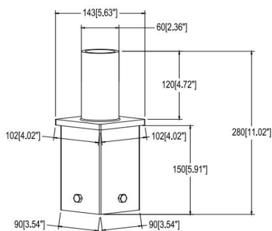
SU-SB-ACC-SQBP-1
